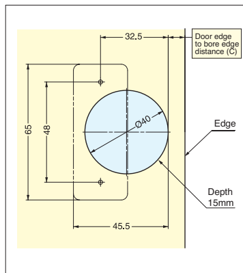
Bore Dimensions
